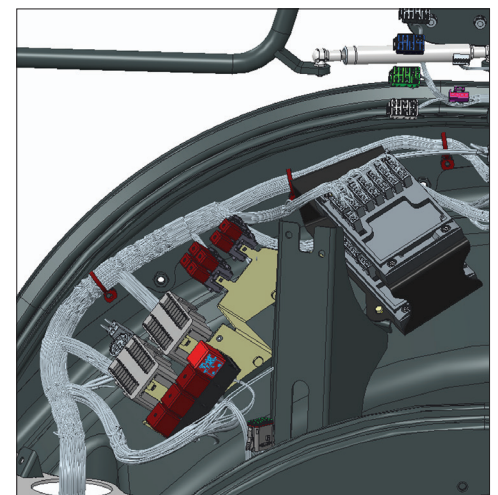
Above, a screenshot of part of the cab harness in the mechanical designers CAD environment. From-to connectivity data (along with connector names) is imported from E 3 .schematic, and the engineer defines routes for the cables to follow. It is in this 3D environment that the cables have mechanical properties (e.g. wire diameters) and that the harness is dressed with clips.
