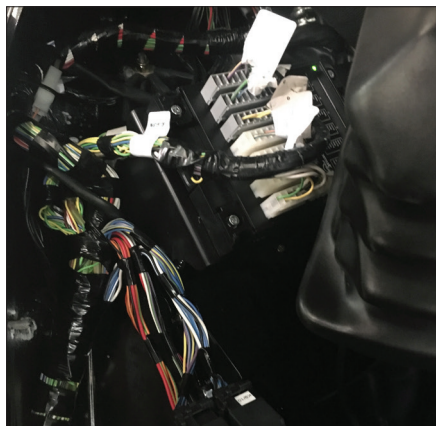
Though designed to fit several vehicle derivatives, the vehicle harnesses are regularly updated to accommodate new vehicle features.
