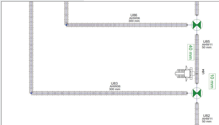
Above, part of cable diagram from E 3 .formboard, showing lengths of conduit (U83, for example), two covered joints (the two green triangles in circles) and the location of fir-tree clips. Full scale (1:1) drawings, which include keys and manufacturer notes, are currently sent to Mecalac's supplier as PDFs for quoting purposes. However, the process will soon become digital to greatly reduce the time taken to receive quotes and, by extension, harnesses back from the supplier.
