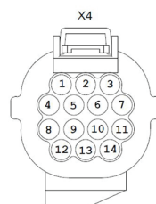
Above, connector information shown in E 3 .formboard. Connectors are all to scale and terminal selection is automatic.
